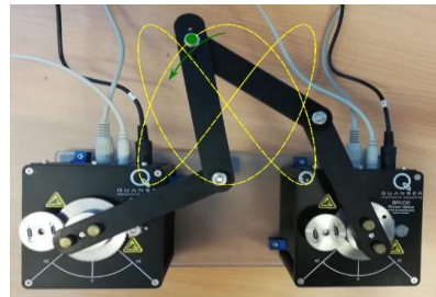
Fig. 10 Two-degree-of-freedom closed-loop robotic system
