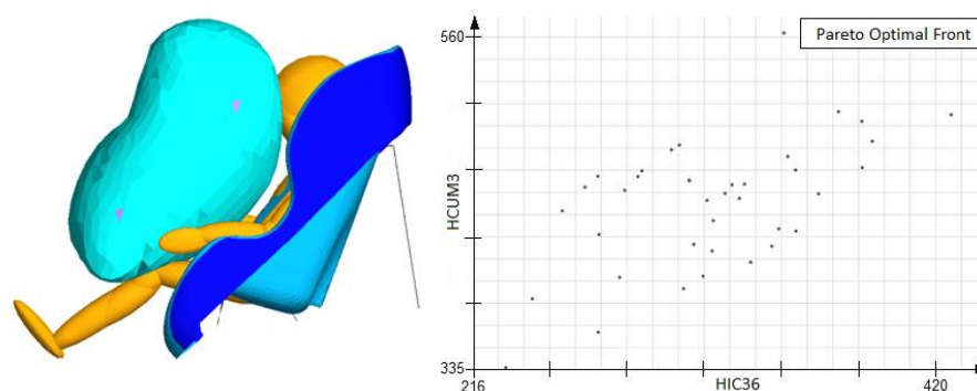
Fig. 19 The intelligent safety belts integrated with the child restraint system with pretensions', load limiters and the airbag (left) and Pareto optimal solution (right)
