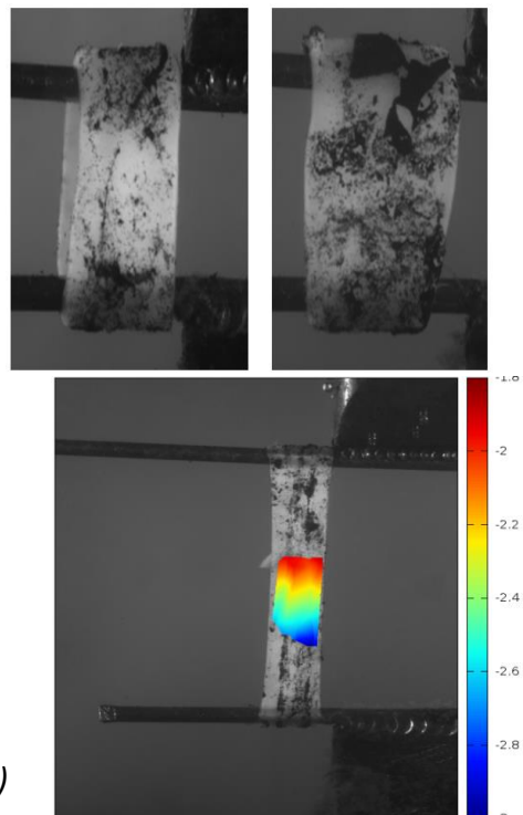
Experimental testing (DIC strain measurement)
